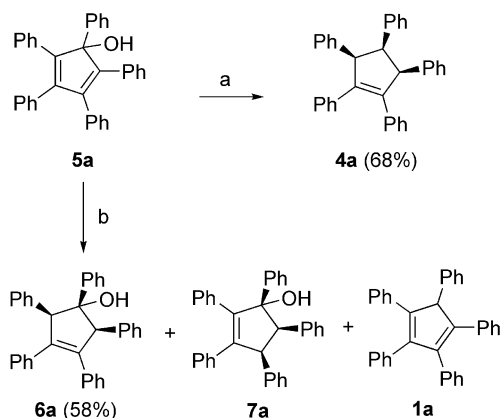
Scheme 3. Catalytic hydrogenation of cyclopentadienol 5a to cyclopentene 4a and cyclopentenols 6a and 7a , respectively. Reagents and conditions: a) Raney nickel, H 2 , 3 bar, 2 d, EtOAc/MeOH 5:1; b) Pd/C, H 2 , 3 bar, 2 d, EtOAc/MeOH 7:1.
