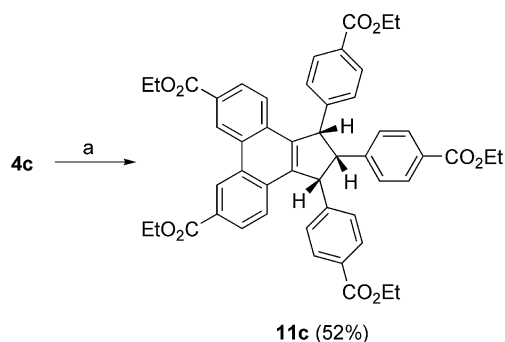
Scheme 6. Photochemical oxidation of cyclopentene 4c to phenanthrene 11c . Reagents and conditions: a) hν , I 2 , N 2 , toluene, 24 h.
