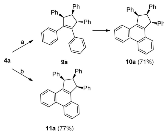
Scheme 5. Formation of the epimeric phenanthrenes 10a and 11a from cyclopentene 4a . Reagents and conditions: a) hν , I 2 , Ar, toluene, 33 h; b) hν , air, toluene, 33 h. The radical-driven formation of 9a precedes the photocyclization–oxidation to 10a .
