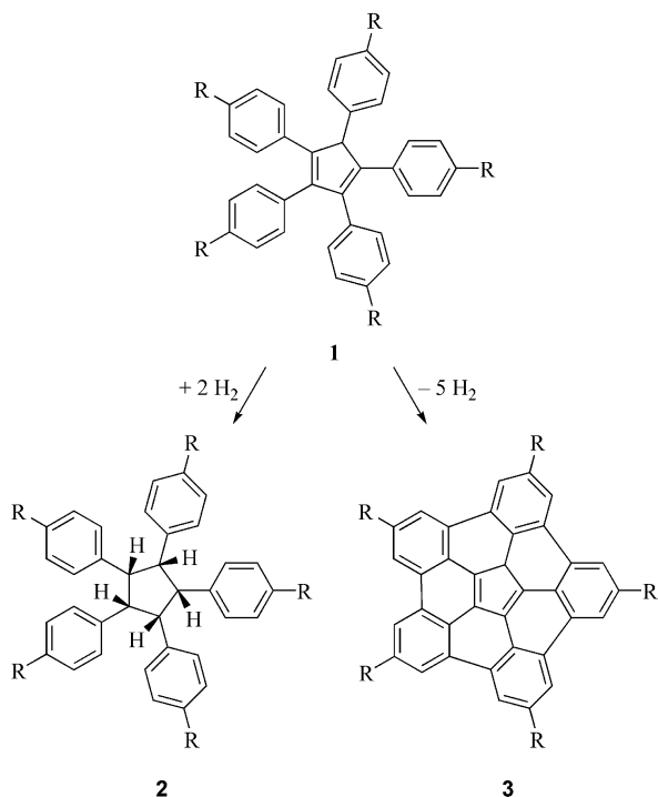
Scheme 1. Spherical target structures 2 and 3 from the reduction and oxidation of cyclopentadiene 1 .
