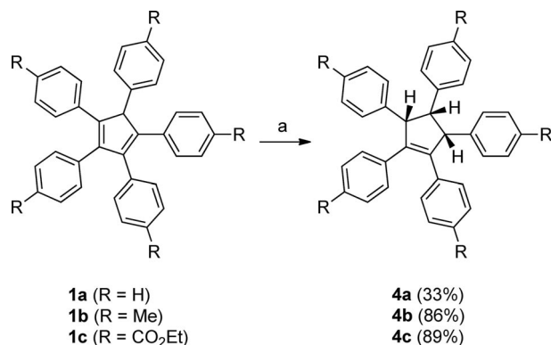
Scheme 2. Catalytic hydrogenation of cyclopentadienes 1a–c . Reagents and conditions: a) Pd/C, H 2 , 3 bar, 2 d, EtOAc ( 4b and 4c ), EtOAc/CHCl 3 ( 4a ), 7 d. The yield of 4a was estimated by 1 H NMR spectroscopy.
