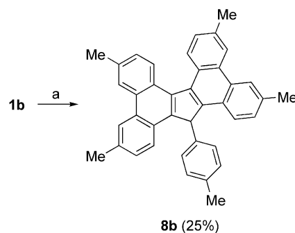
Scheme 4. Cyclodehydrogenation of cyclopentadiene 1b to bis-phenanthrene 8b . Reagents and conditions: a) AlCl 3 /CuCl 2 , CS 2 , room temperature, 5 min.
