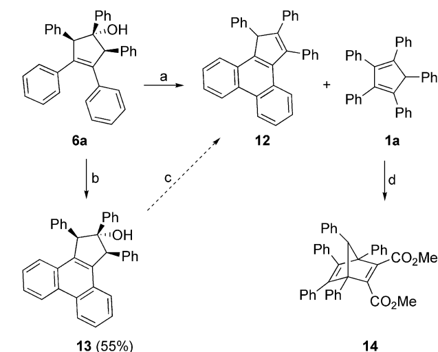
Scheme 7. Formation of phenanthrenes 12 and 13 from cyclopentenol 6a in the presence and absence of oxygen, respectively. The transformation d is necessary for the separation of 12 and 1a . Reagents and conditions. a) hν , MeOH, I 2 , Ar, 22 h; b) hν , toluene, O 2 , 68 h; c) hν , MeOH, I 2 , Ar, 6a ; d) dimethyl acetylenedicarboxylate, toluene, 110 °C, 16 h.
